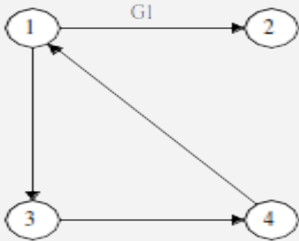
(a) G1
